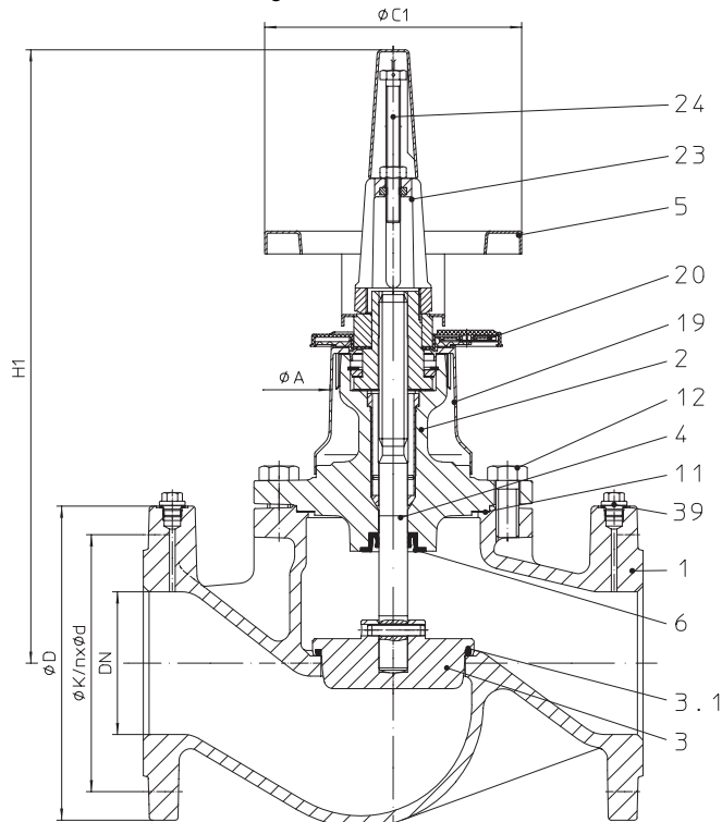
Fig 12.020 DN 15 - 80
